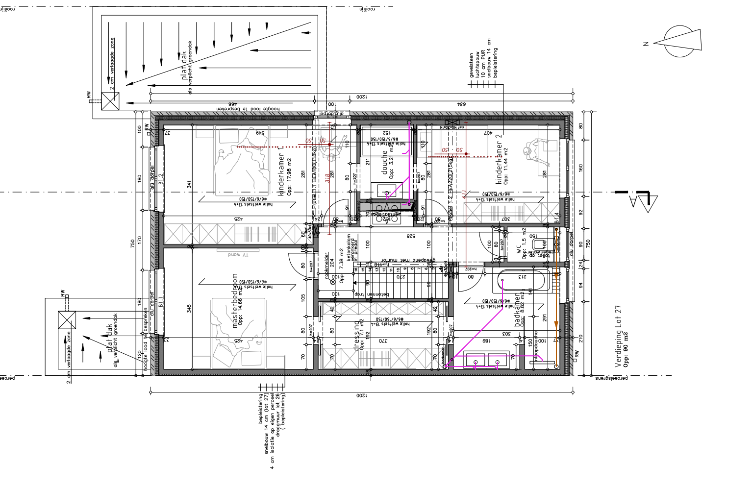
Verdieping Lot 27 Opp: 80 m 2
